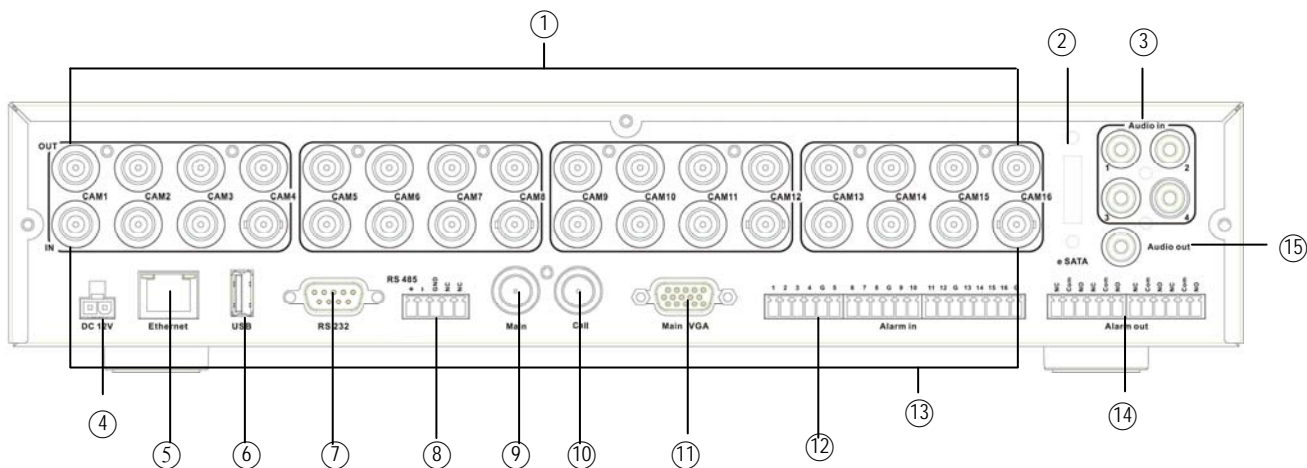
Figure 1-2 Rear Panel
