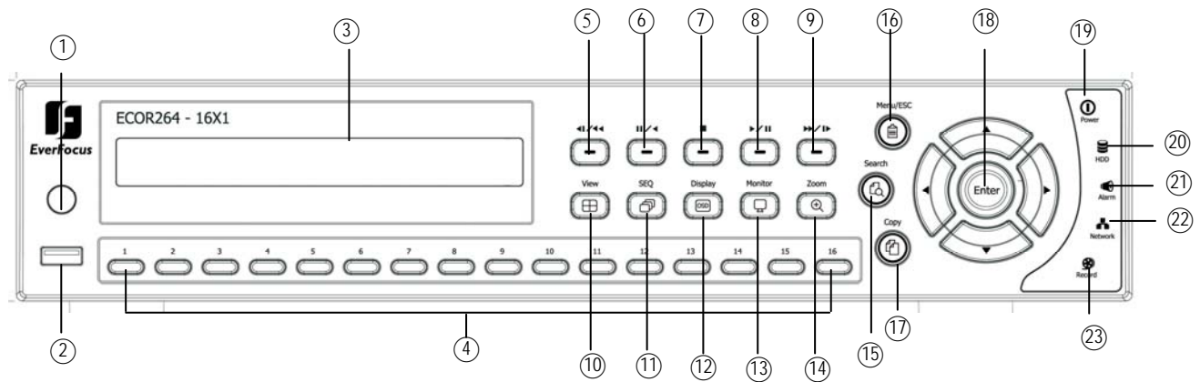
Figure 1-1 Front Panel
